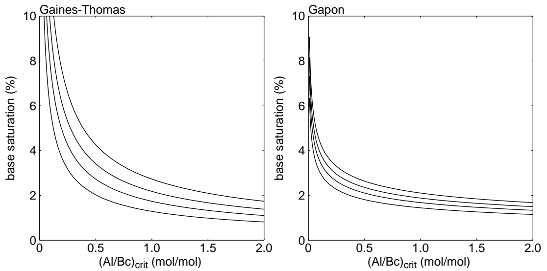
Figure B: Base saturation as a function of the (critical) molar Al/Bc-ratio for 4 different base cation concentrations ( [Bc]=20 (lowest curve), 50, 100 and 200 meq/L (highest curve); \alpha=3 and KAl_{ox}=10^8 (mol/L) ^{-2} ). (a) For the Gaines-Thomas exchange equations ( K_{AlBc}=1 mol/L, K_{HBc}=10^5 (mol/L) ^{-1} ), and (b) for Gapon exchange equations ( k_{AlBc}=10 (mol/L) ^{1/6} , k_{HBc}=10 (mol/L) ^{-1/2} ).
