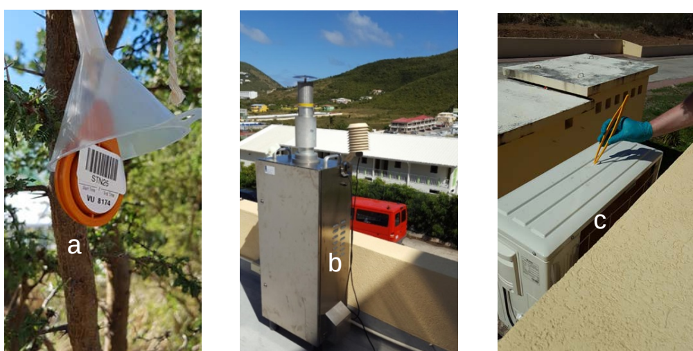
Figure 1. 3M badge for passive sampling at location 1 (a), Leckel filter equipment at location D (b) and swiping dust for historical interpretation (c).
