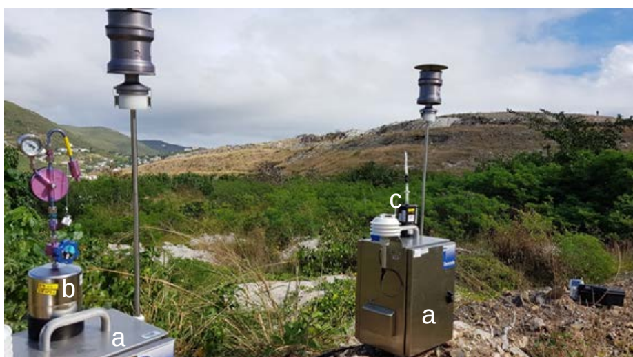
Figure 2. Two KFG dust samplers (a), canister (b) and pump with sorbent tube (c) at VROMI yard (location 4).
