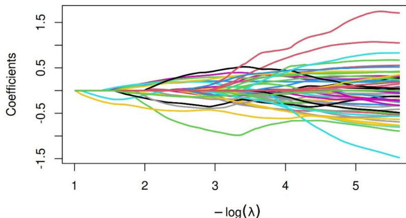
Figure A3 LASSO coefficient paths as a function of the regularisation parameter.
