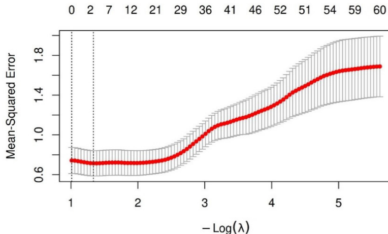
Figure A2 Selection of the optimal regularisation parameter lambda ( \lambda ) in LASSO regression using 10-fold cross-validation.
