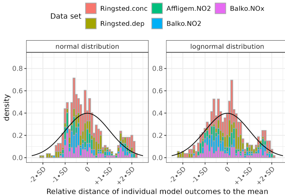
Figure 6.6 Distribution of individual model outcomes in the current study. Left-hand pane: distribution of (\text{outcome}-\text{AM})/\text{SD} , right-hand pane: distribution of \log_{\text{GSD}}((\text{outcome}/\text{GM})) .
