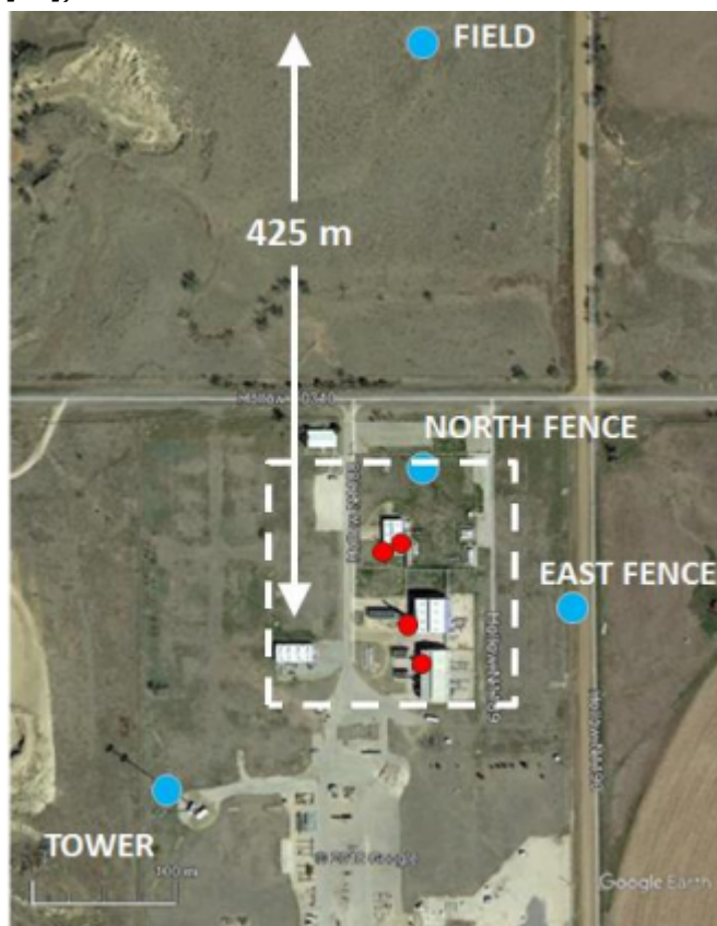
Figure 5.1 Top view of the release locations (red circles) and concentration monitors (blue circles) at the Balko compressor station (image copied from [25]).
