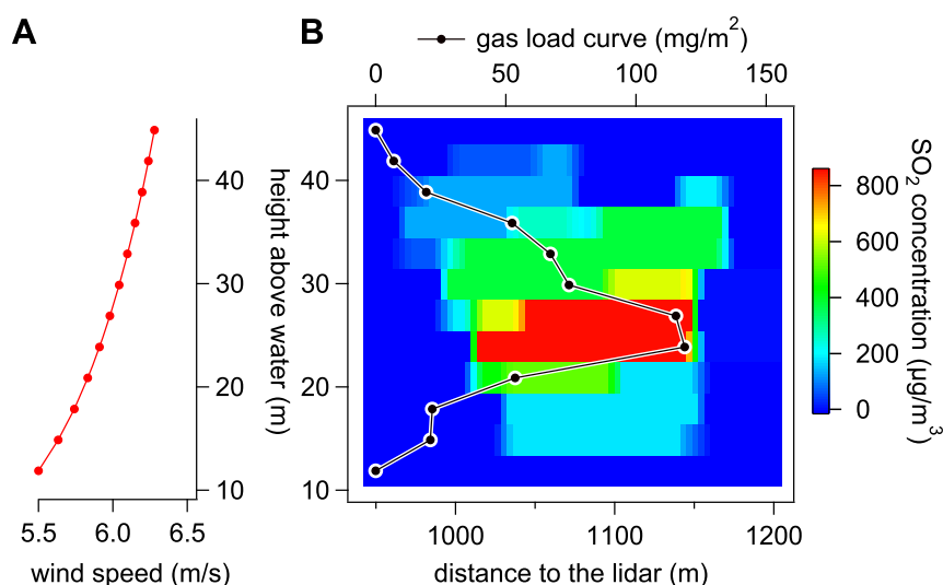
Figure 2-10 A : logarithmic wind profile; B : cross-section from Figure 2-9 of the smoke plume of the HMS Rotterdam, and the corresponding gas load curve
