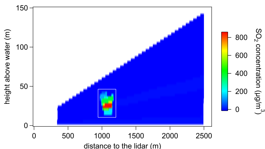
Figure 2-9. Cross section through the smoke plume of the HMS Rotterdam. The colour indicates the concentration of \text{SO}_2 in the air. The white rectangle shows the plume as it was used in the further analysis.
