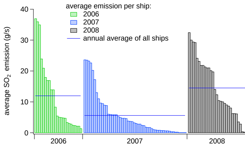
Figure 3-1. The historical development of the emissions Each vertical bar represents a ship for which an average emission value was measured. For each year the emissions are sorted into a declining order. For each year the average emissions for all ships measured that year are shown.
