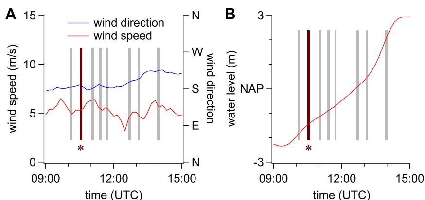
Figure 2-11. Wind and water data at Hansweert, measured by Rijkswaterstaat, on 9 October 2006
