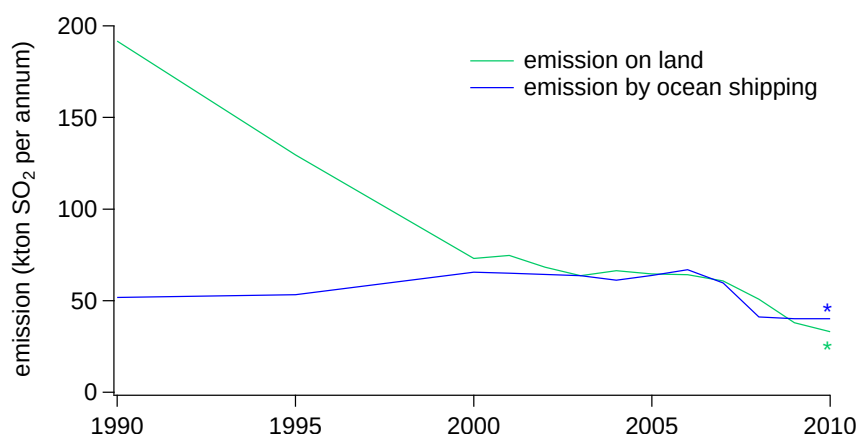
Figure 1-1. The development of sulphur dioxide emissions between 1990 and 2010
