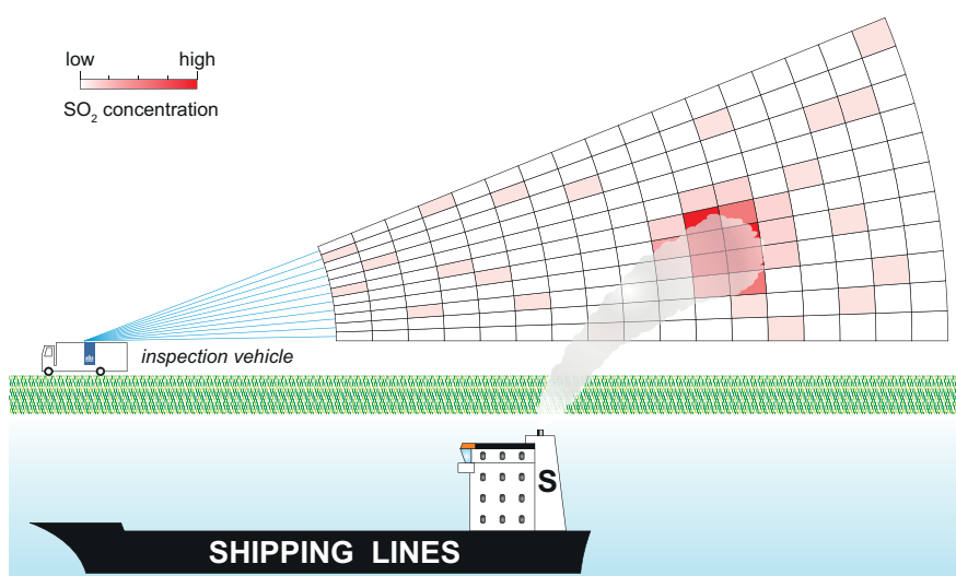
Figure 2-3. Side view of the situation during an emission measurement
