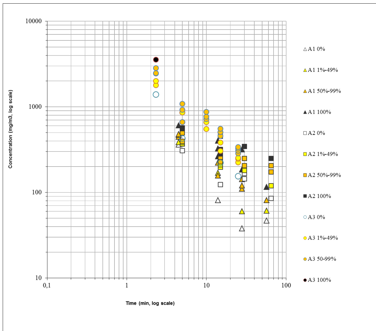
1 2 Figure 4 Final data selected for derivation of the animal probit function of hydrogen 3 cyanide (identical to figure 2). 4 5
