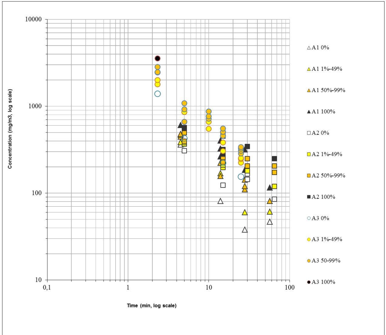
Figure 2 Data selected for the initial analysis for the derivation of the animal probit function of hydrogen cyanide
