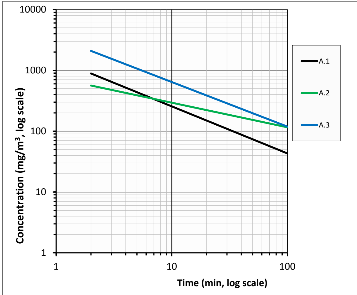
Figure 3 LC 50 values of A study datasets for hydrogen cyanide, over time where available.
