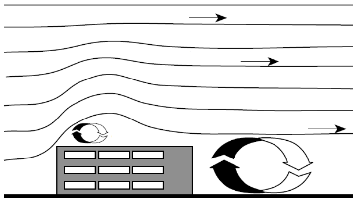
Figure 4.8. Sketch of effect of building on streamlines around the building. From Scholten et al. (1998).
