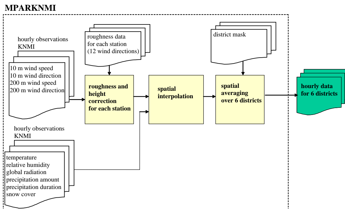
Figure 2.3 Processing of primary meteorological data by MPARKNMI.
