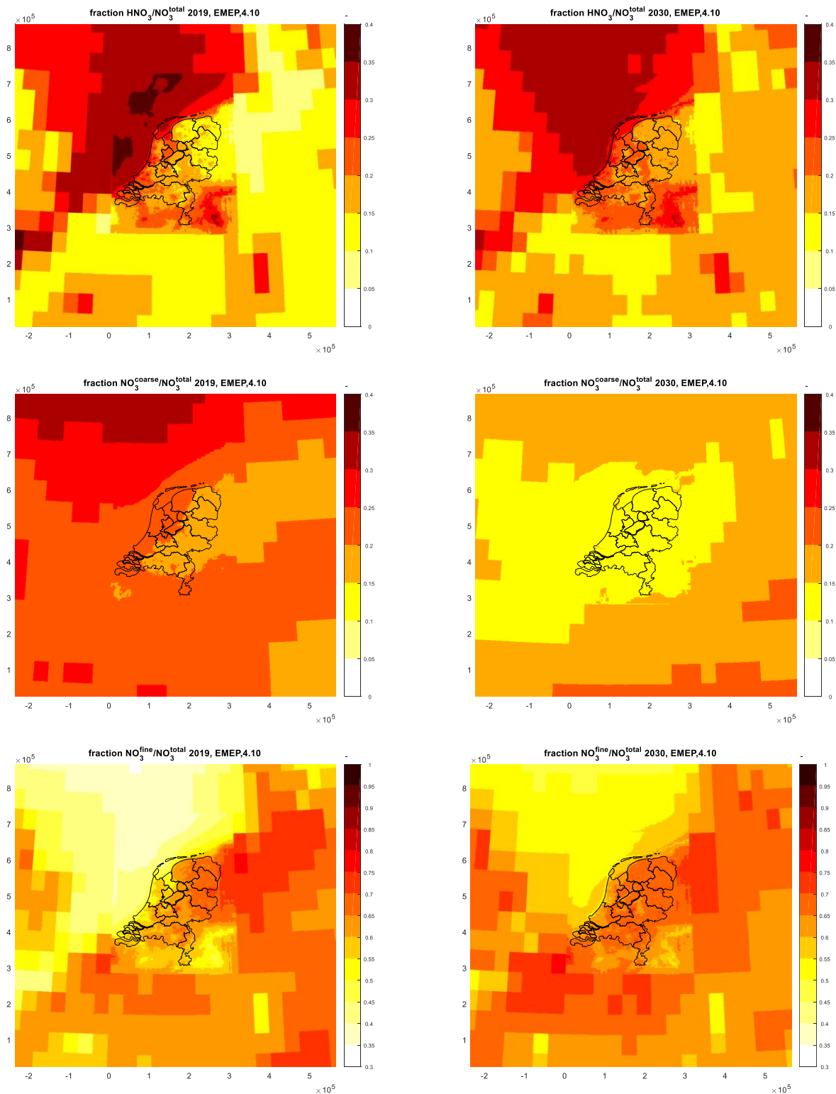
Figure 7.6. Yearly averaged fractions of sub-species of \text{NO}_3^{\text{total}} from EMEP for 2019 (left panels) and 2030 (right panels). Top row: \text{HNO}_3/\text{NO}_3^{\text{total}} ; (range [0 0.4]), middle row: \text{NO}_3^{\text{coarse}}/\text{NO}_3^{\text{total}} (range [0 0.4]), bottom
