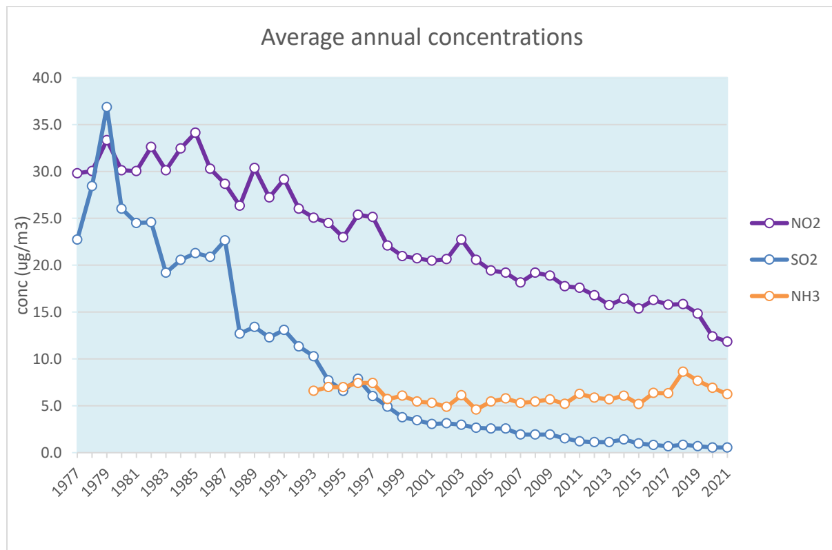
Figure 7.10. Average annual concentrations ( \mu\text{g}/\text{m}^3 ) of \text{SO}_2 , \text{NO}_2 and \text{NH}_3 , derived from measurements at the regional stations of the LML network. For \text{NH}_3 also stations of the MAN network are used starting in 2005. See table 7.4 for representative periods.
