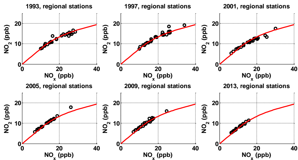
Figure 7.8: Yearly averaged \text{NO}_2 - vs. \text{NO}_x -concentration for regional LML-stations. In red the \text{NO}_x \rightarrow \text{NO}_2 -conversion function.
