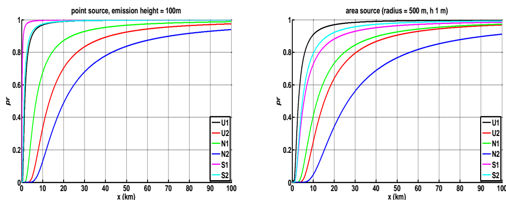
Figure 6.4: Distributing factor pr (according to Eq. 6.12) between below-cloud and in-cloud scavenging as function of source-receptor distance x for different meteo classes U : unstable, N : neutral, S : stable. \sigma_z computed as a x^b , (see eq. 3.18), mixing height as in Table 2.5). pr = 0 \rightarrow below cloud scavenging, pr = 1 \rightarrow in-cloud scavenging. Left panel: point source with emission height 100 m, right panel: area source with emission height of 1 m. Note that in the case of a point source in meteo class S1 , the emission is above the mixing height.
